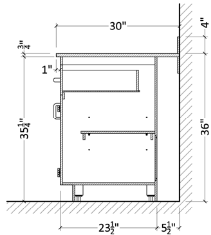
TYPICAL CABINET SECTION
